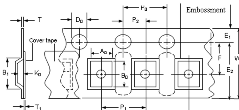
EIA Tape Component Dimentions
