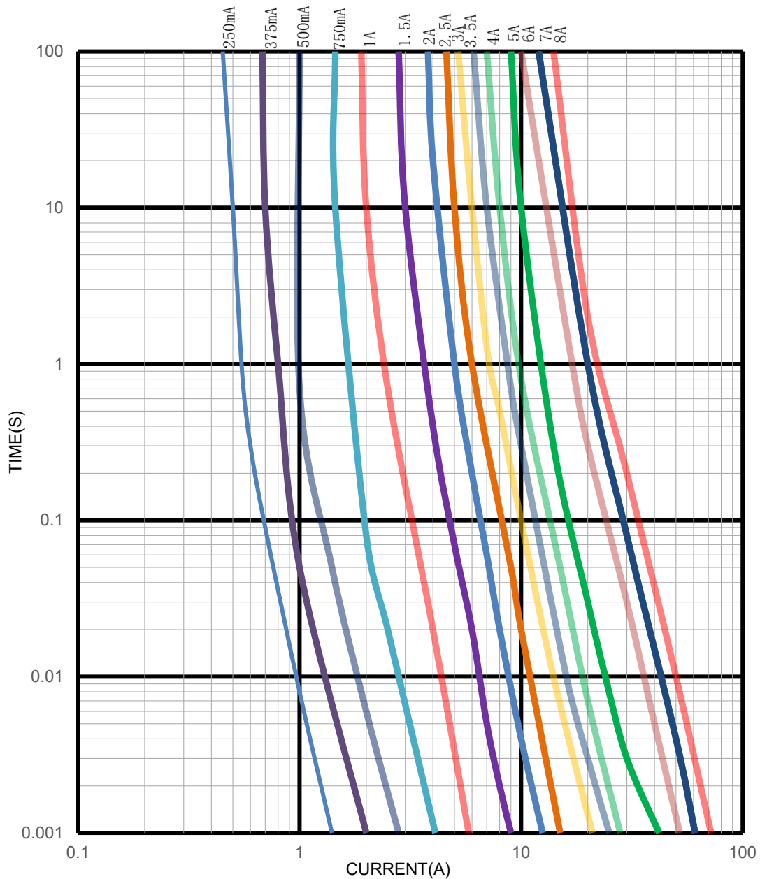
Time-Current Curve
