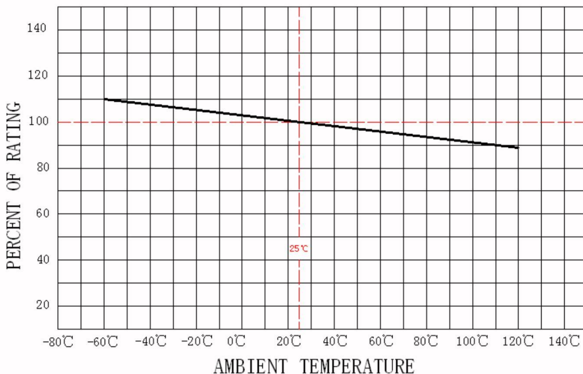
Temperature-Current curve:
