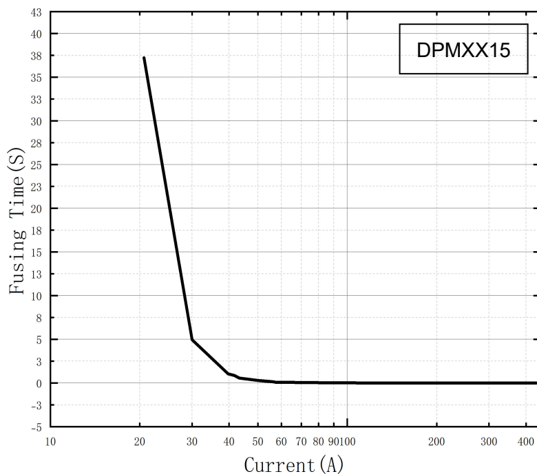
5-2 2倍I-t图/CHARACTERISTICS DIAGRAM(2*I-t)
