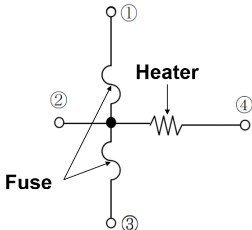
等效电路/ Equivalent Circuit
